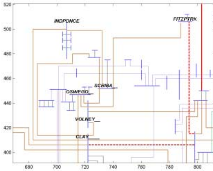
Figure 7c: A Simulated Cascading Disturbance in NYPP
