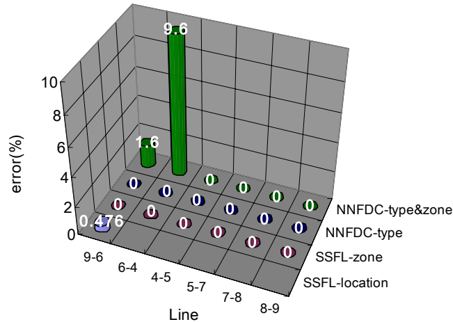
Figure 3.20 Classification and location error of test #2
