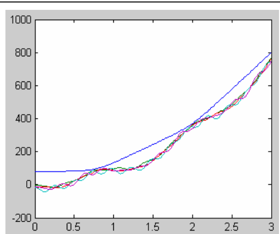
Figure 2.9 Machine angles when 24.5% load shedding at t=0.11s
