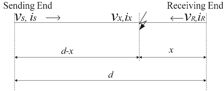
Figure 3.3 A faulted transmission line
