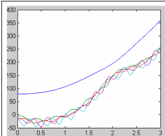
Figure 2.8 Machine angles when 5.5% load shedding at t=0.11s
